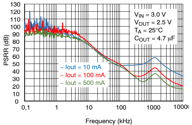
Figure 25. Power Supply Rejection Ratio for V_{OUT} = 2.5 \text{ V} , C_{OUT} = 4.7 \mu\text{F}
