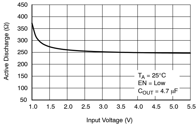
Figure 24. Active Discharge Resistance vs. Input Voltage
