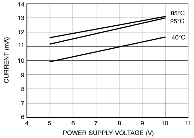
Figure 18. Supply Current vs. Power Supply Voltage (Enabled)
