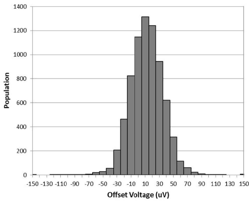
Figure 3. Input Offset Production Distribution G200
