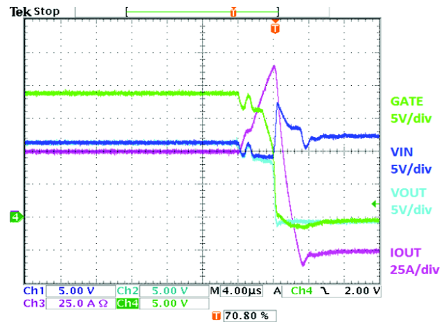
Figure 29. Short Circuit during Normal Operation ( I_{out} = 50\text{ A} )
