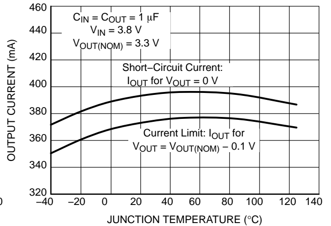
Figure 32. Short-Circuit Limit vs. Temperature V_{OUT} = 3.3 \text{ V}
