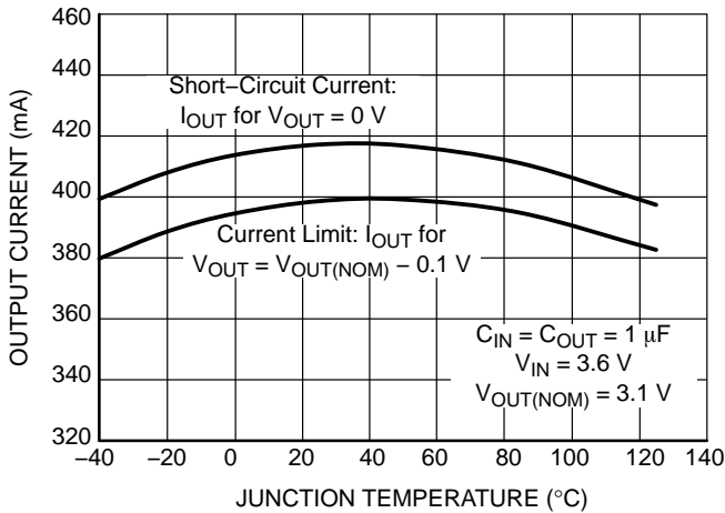
Figure 31. Short-Circuit Limit vs. Temperature V_{OUT} = 3.1 \text{ V}
