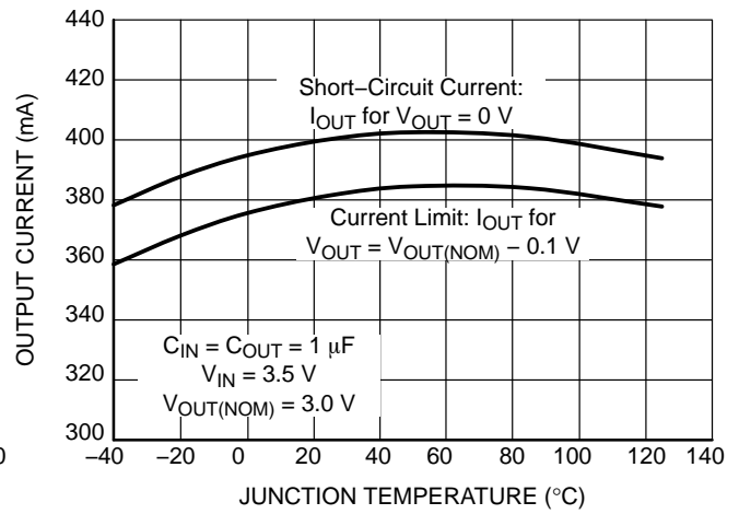
Figure 30. Short-Circuit Limit vs. Temperature V_{OUT} = 3.0 \text{ V}
