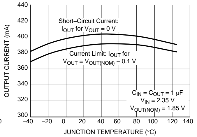
Figure 28. Short-Circuit Limit vs. Temperature V_{OUT} = 1.85 \text{ V}
