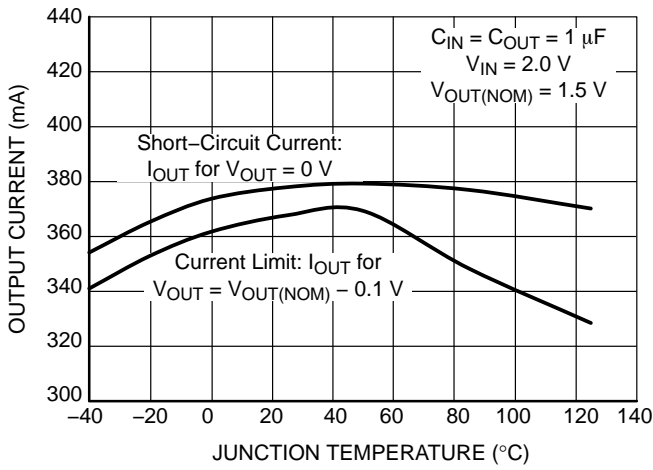
Figure 27. Short-Circuit Limit vs. Temperature V_{OUT} = 1.5 \text{ V}
