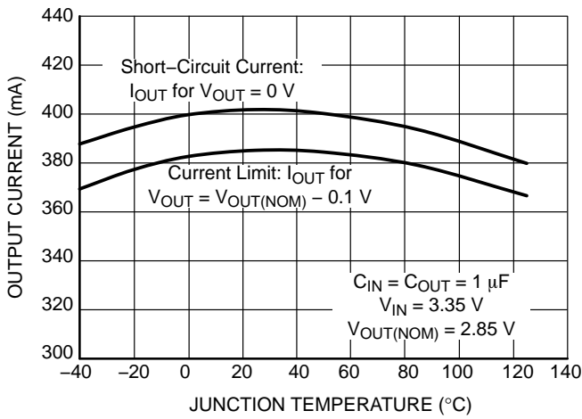
Figure 29. Short-Circuit Limit vs. Temperature V_{OUT} = 2.85 \text{ V}
