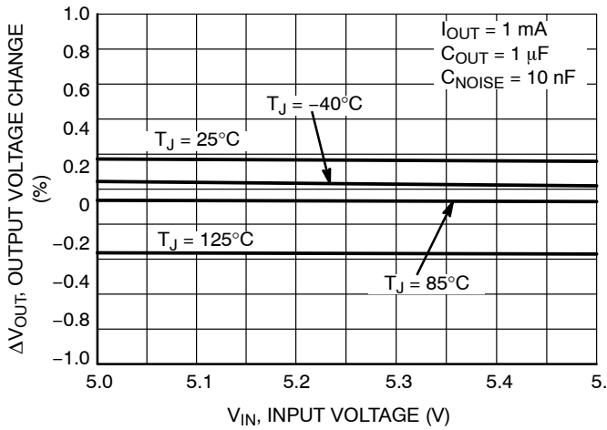
Figure 5. Line Regulation
