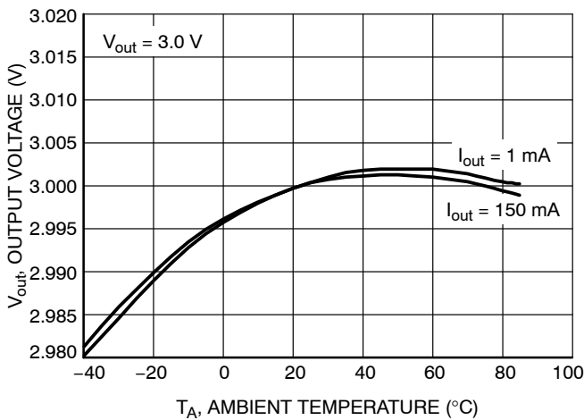
Figure 7. Output Voltage vs. Temperature ( V_{out} = 3.0 V)
