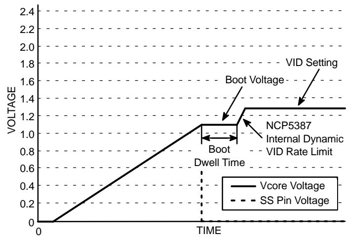
Figure 27. Typical VR10 & VR11 Soft-Start Sequence to Vcore = 1.3 V
