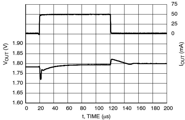
Figure 55. Load Transients, 1.8 V Version, I_{OUT} = 1 - 50 mA, t_R = t_F = 0.5 \mu s, V_{IN} = 2.8 V, AE = 0 V
