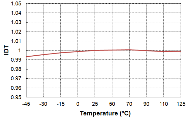
Figure 4. I_{DT} vs. Temperature
