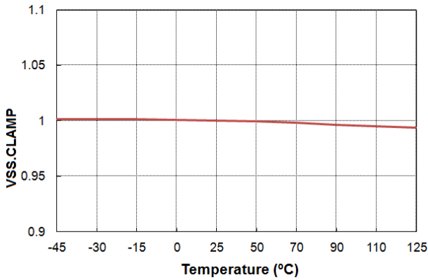
Figure 11. VSS.CLAMP vs. Temperature
