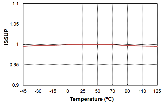
Figure 31. I SS,UP vs. Temperature
