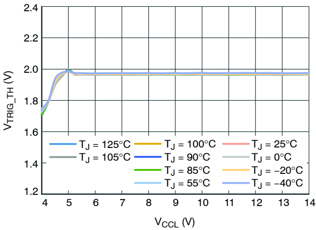
Figure 28. Trigger Threshold
