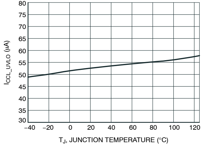
Figure 15. VCCL Current Consumption Below UVLO, V_{CC} = V_{CCLOFF} - 0.1 V
