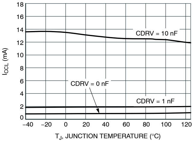
Figure 18. VCCL Current Consumption for 10 V Driver, V_{CS} = -1 to 4 V, f_{CS} = 100 kHz, V_{CC} = 12 V
