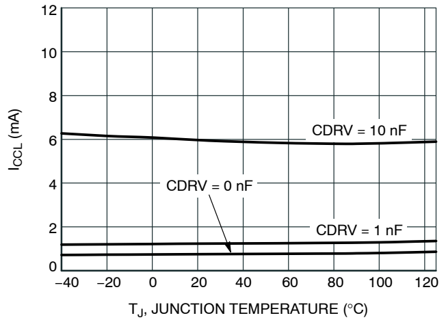
Figure 19. VCCL Current Consumption for 5 V Driver, V_{CS} = -1 to 4 V, f_{CS} = 100 kHz, V_{CC} = 12 V
