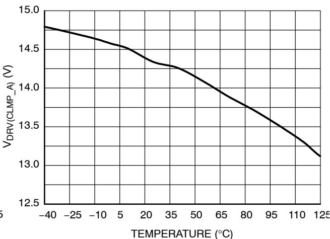
Figure 16. Driver Clamp Level – A Version, V_{CC} = 28\text{ V} and C_{DRV} = 10\text{ nF}
