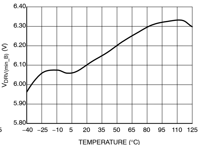
Figure 14. Minimal Driver High Level – B Version, V_{CC\_off} + 0.2\text{ V} and C_{DRV} = 0\text{ nF}
