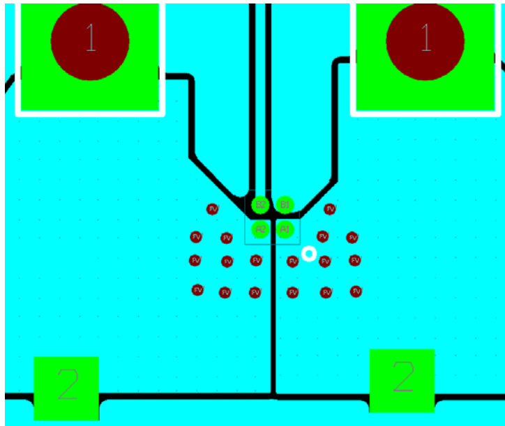
Figure 13. Routing Example 1 oz, 2 Layers, 100 ^{\circ}C/W
