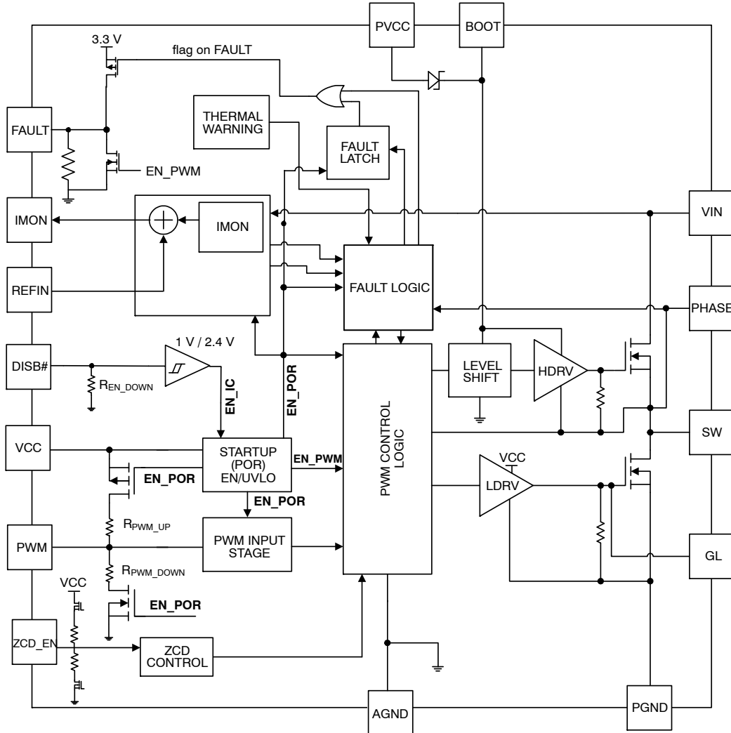
Figure 2. Block Diagram
