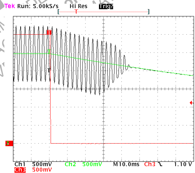
Figure 41. TurningOff Time Zoom/ V_p = 5.0\text{ V} and F = 400\text{ Hz} Ch1 = OUT_R, Ch2 = VMC and Ch3 = Shutdown
