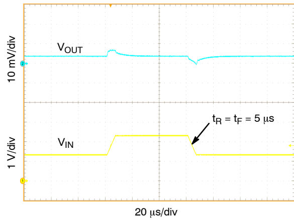
Figure 19. V_{IN} Line Transient Response, V_{IN} = 1.3\text{ V to } 2.3\text{ V} , I_{OUT} = 100\text{ mA} , C_{OUT} = 2.2\ \mu\text{F}
