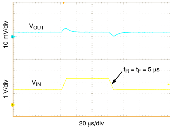
Figure 18. V_{IN} Line Transient Response, V_{IN} = 1.3\text{ V to } 2.3\text{ V} , I_{OUT} = 100\text{ mA} , C_{OUT} = 10\ \mu\text{F}
