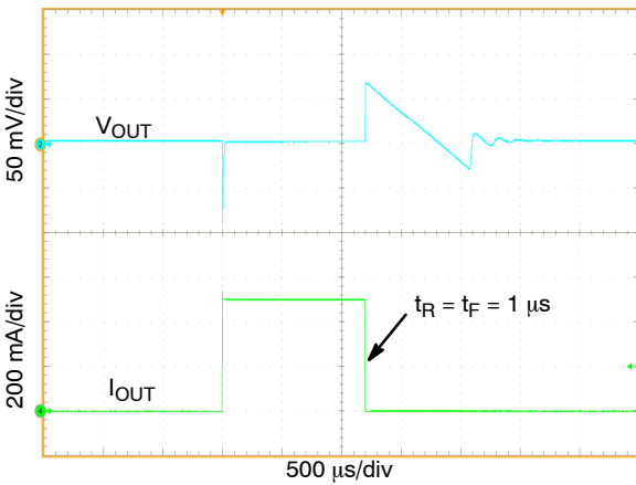
Figure 14. Load Transient Response, I_{OUT} = 1\text{ mA} to 500\text{ mA} , C_{OUT} = 10\text{ }\mu\text{F}
