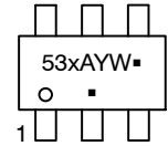
TSOP-6 CASE 318G STYLE 13
