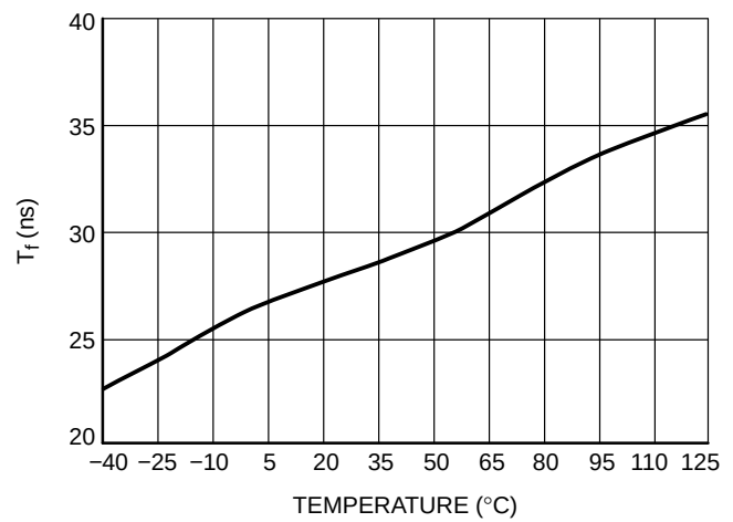
Figure 28. Output Voltage Fall-time, T f
