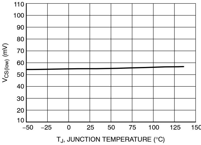
Figure 34. Current Sense Lower Threshold (V CS Falling) vs. Temperature
