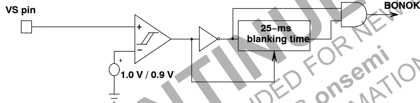
Figure 69. Brown-out Circuit
