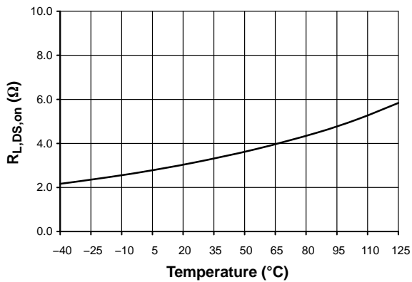
Figure 25. On-State Resistance of the Driving NMOS, R L,DS,on
