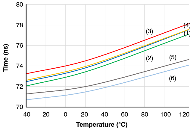
(1) t_{PD-OFF-A}, V_{DD1} = 3.3V (2) t_{PD-OFF-B}, V_{DD1} = 3.3V (3) t_{PD-OFF-A}, V_{DD1} = 5V (4) t_{PD-OFF-B}, V_{DD1} = 5V (5) t_{PD-OFF-A}, V_{DD1} = 20V (6) t_{PD-OFF-B}, V_{DD1} = 20V
