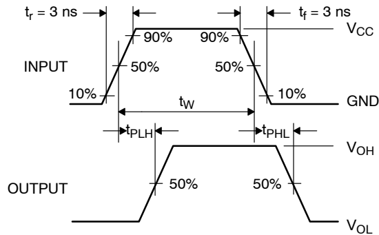
Figure 6. AC Waveforms
