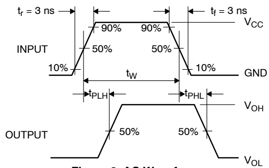
Figure 6. AC Waveforms
