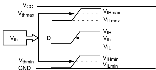
Figure 16. V_{th} Diagram
