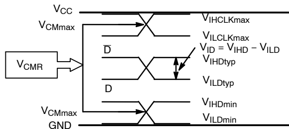
Figure 17. V_{CMR} Diagram
