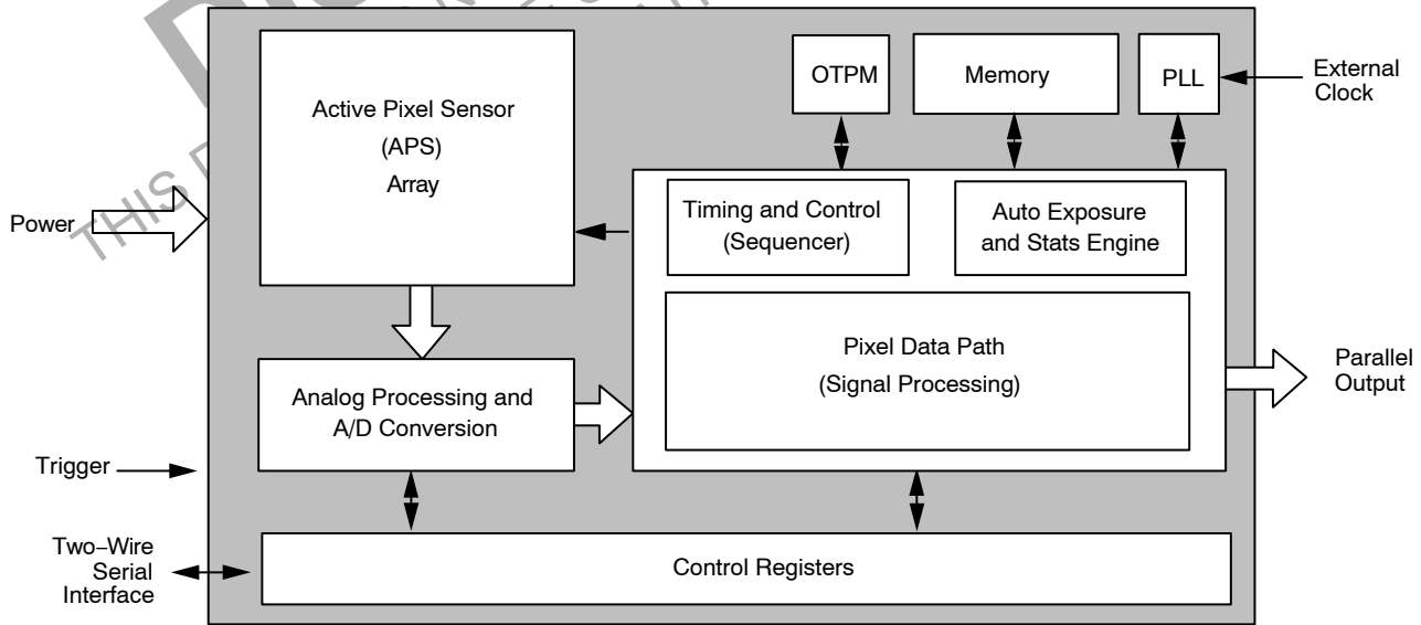
Figure 1. Block Diagram
