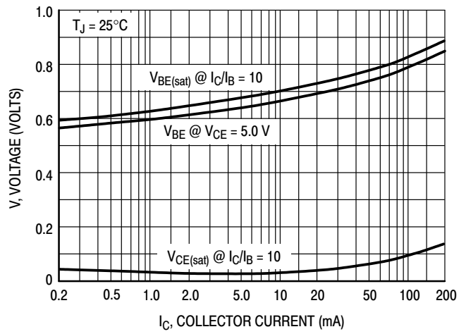
Figure 7. "ON" Voltages
