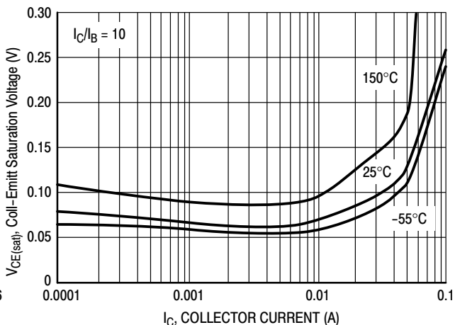
Figure 4. V_{CE(sat)}
