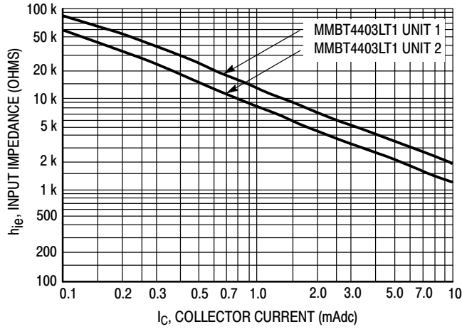
Figure 9. Input Impedance
