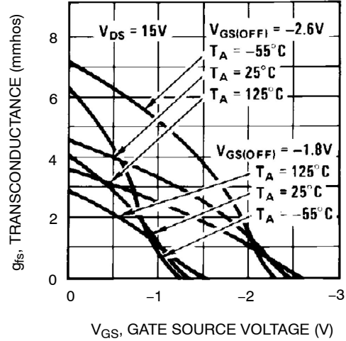
Figure 4. Transfer Characteristics
