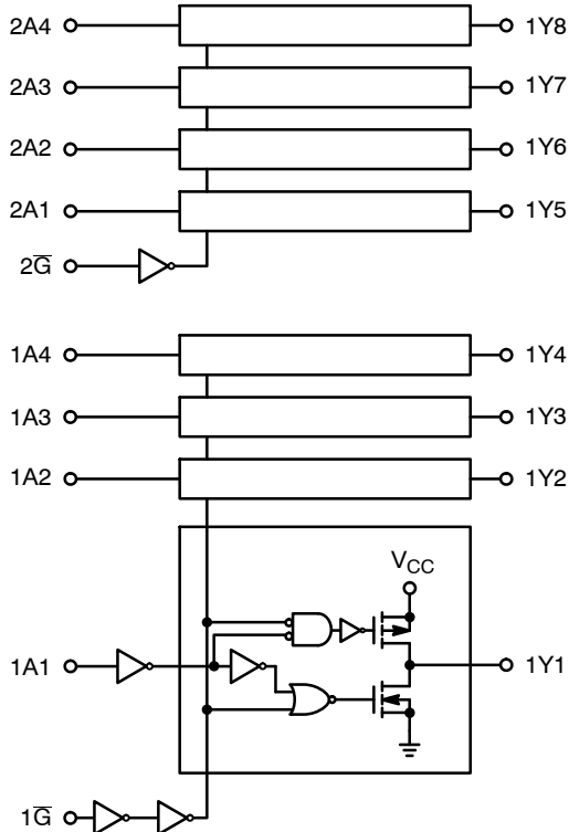
Figure 1. Logic Diagram
