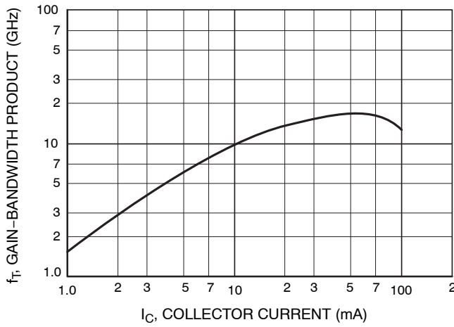
Figure 7. f_T - I_C
