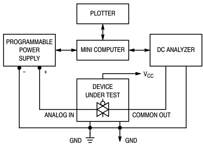
Figure 1. On Resistance Test Set-Up
