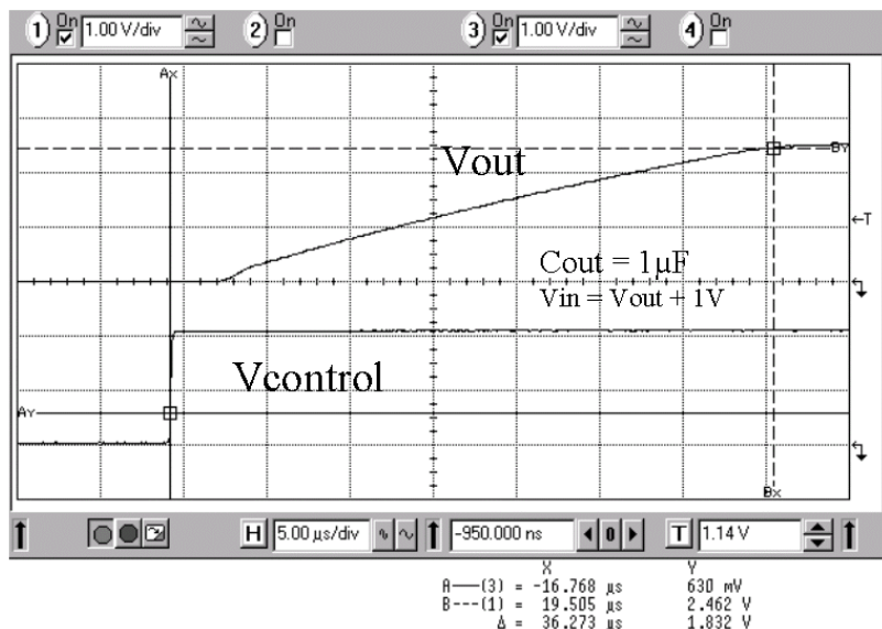
Figure 12. Repetitive Start-Up Waveforms
