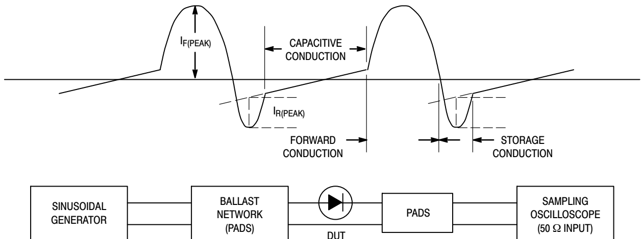
Figure 5. Krakaer Method of Measuring Lifetime
