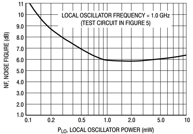
Figure 4. Noise Figure
