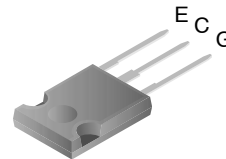
TO-247-3LD SHORT LEAD CASE 340CK JEDEC STYLE
