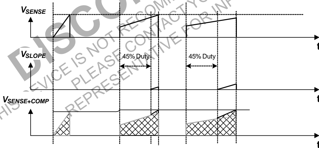
Figure 38. Slope Compensation
