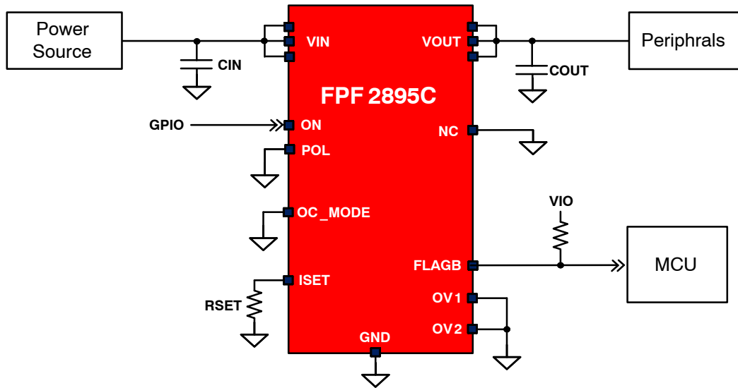
Figure 1. Typical Application
