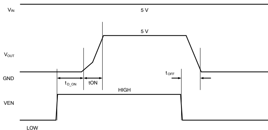
Figure 4. V_{IN} to V_{OUT} Power Up/Down and Normal Operation
