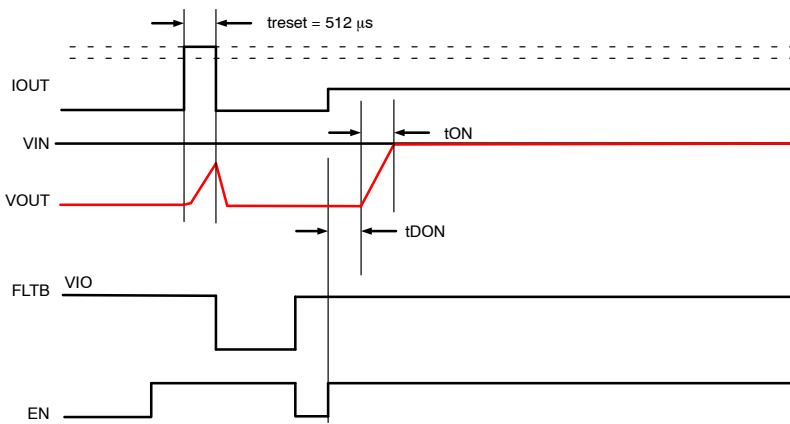
Figure 5. Inrush Current Limit and SCP Operation (Latch-Off)
