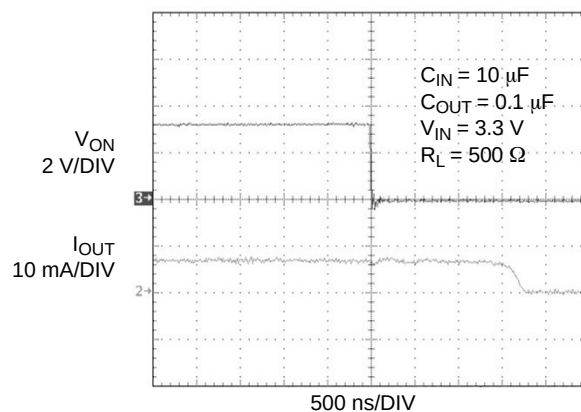
Figure 19. t_{dOFF} Response
