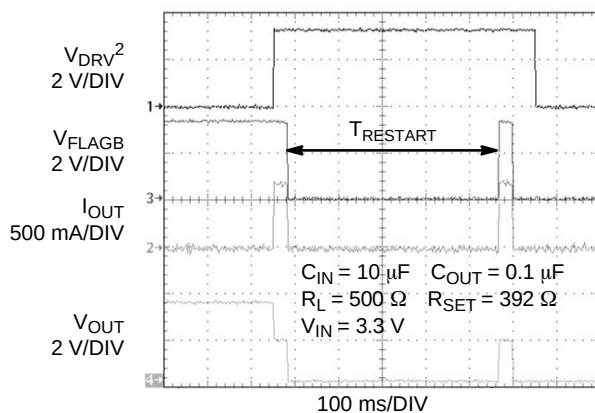
Figure 17. T_{RESTART} Response
