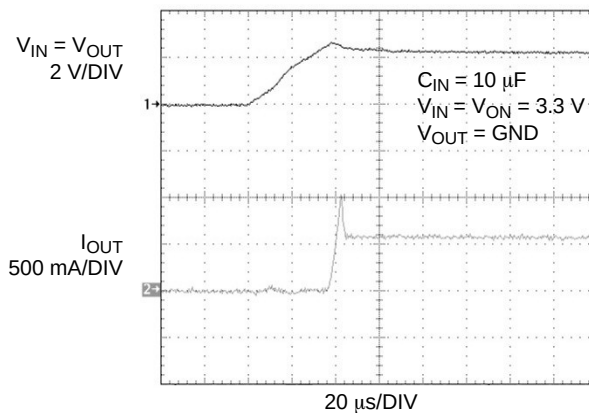
Figure 21. Current Limit Response Time (Switch is Powered into a Short)
