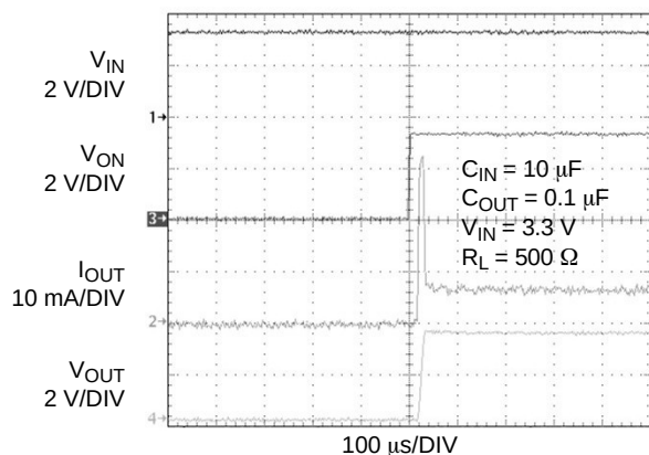
Figure 18. t_{dON} Response
