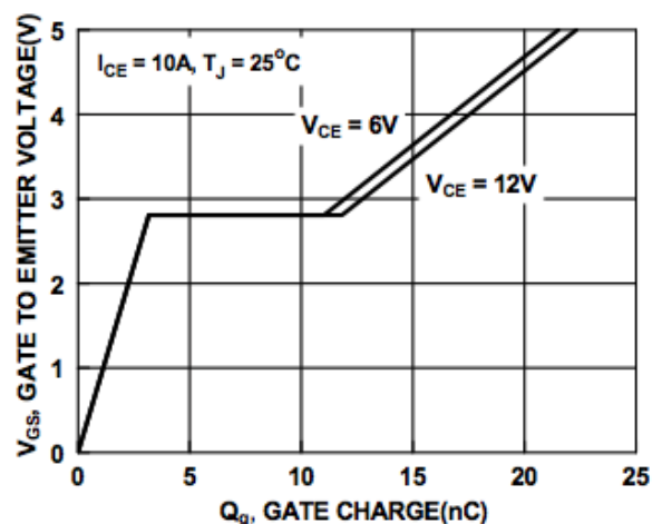
Figure 10. Gate Charge
