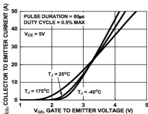
Figure 8. Transfer Characteristics
