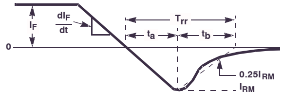
Figure 14. T_{rr} Waveforms and Definitions
