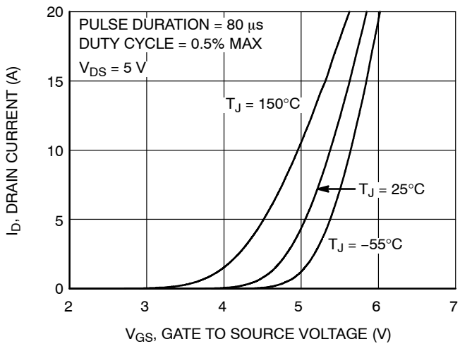
Figure 5. Transfer Characteristics
