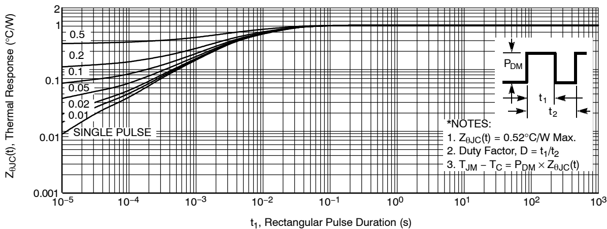
Figure 13. Transient Thermal Response Curve for FDP12N60NZ
