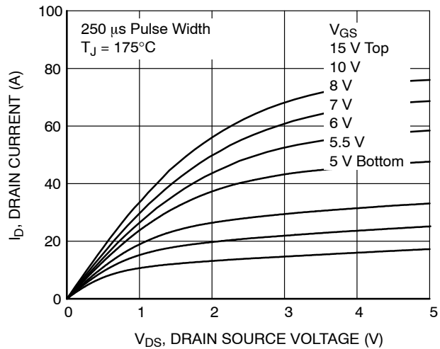
Figure 10. Saturation Characteristics
