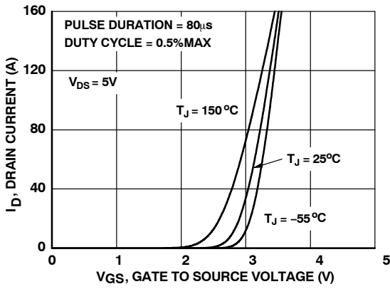
Figure 9. Transfer Characteristics
