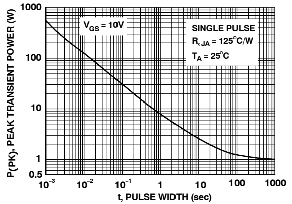
Figure 16. Single Pulse Maximum Power Dissipation
