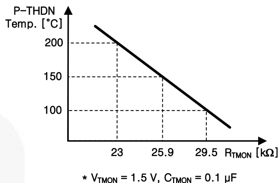
Figure 36. R_{TMON} vs. P-THDN Temperature
