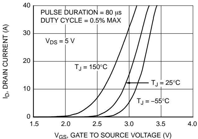
Figure 17. Transfer Characteristics
