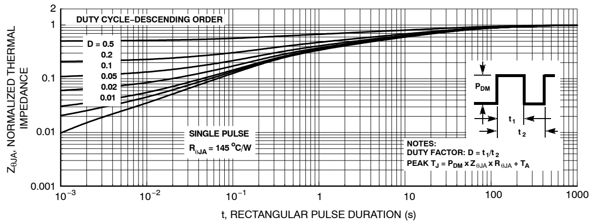
Figure 11. Junction-to-Ambient Transient Thermal Response Curve
